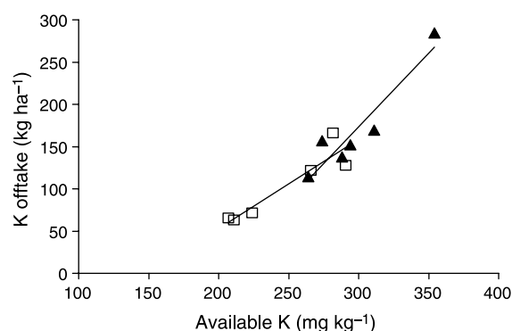
Figure 1. Relationship between the available K (ammonium nitrate extractable) measured in the soil in autumn 1999 and plant K offtake the following year (2000) at SAC (□, r^2 = 0.86 ) and EFRC (▲, r^2 = 0.89 ). For site key, see Materials and Methods.
